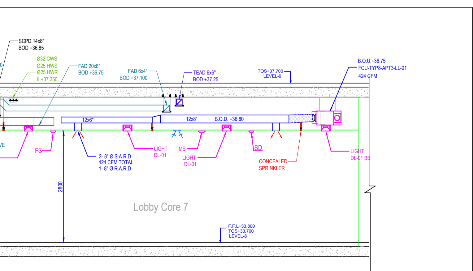
Level 8 H/L - Composite Layout SCALE = 1:50
