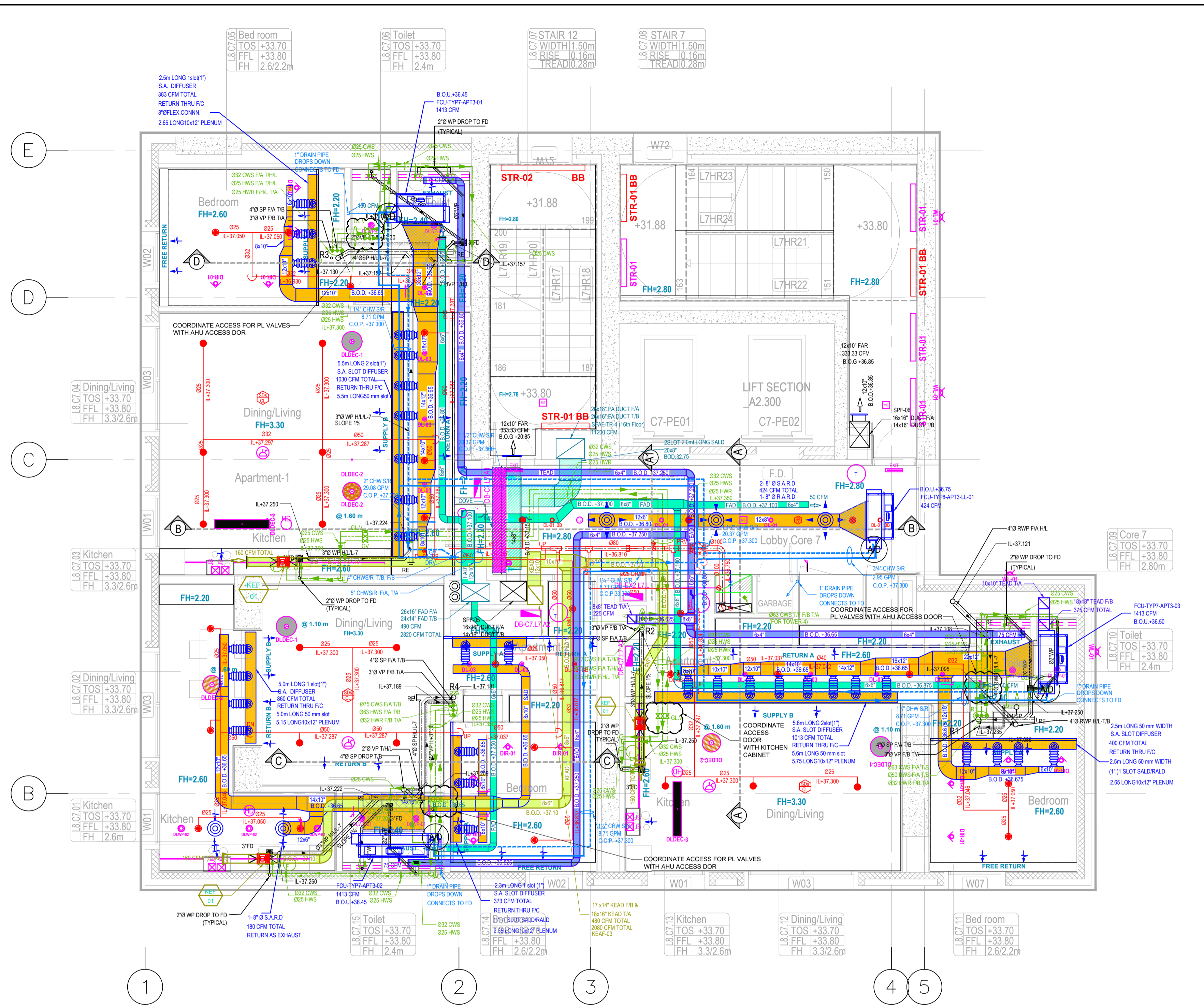
Level 8 H/L - Composite Layout SCALE = 1:50
