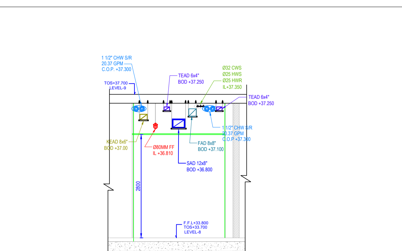
Level 8 H/L - Composite Layout SCALE = 1:50
